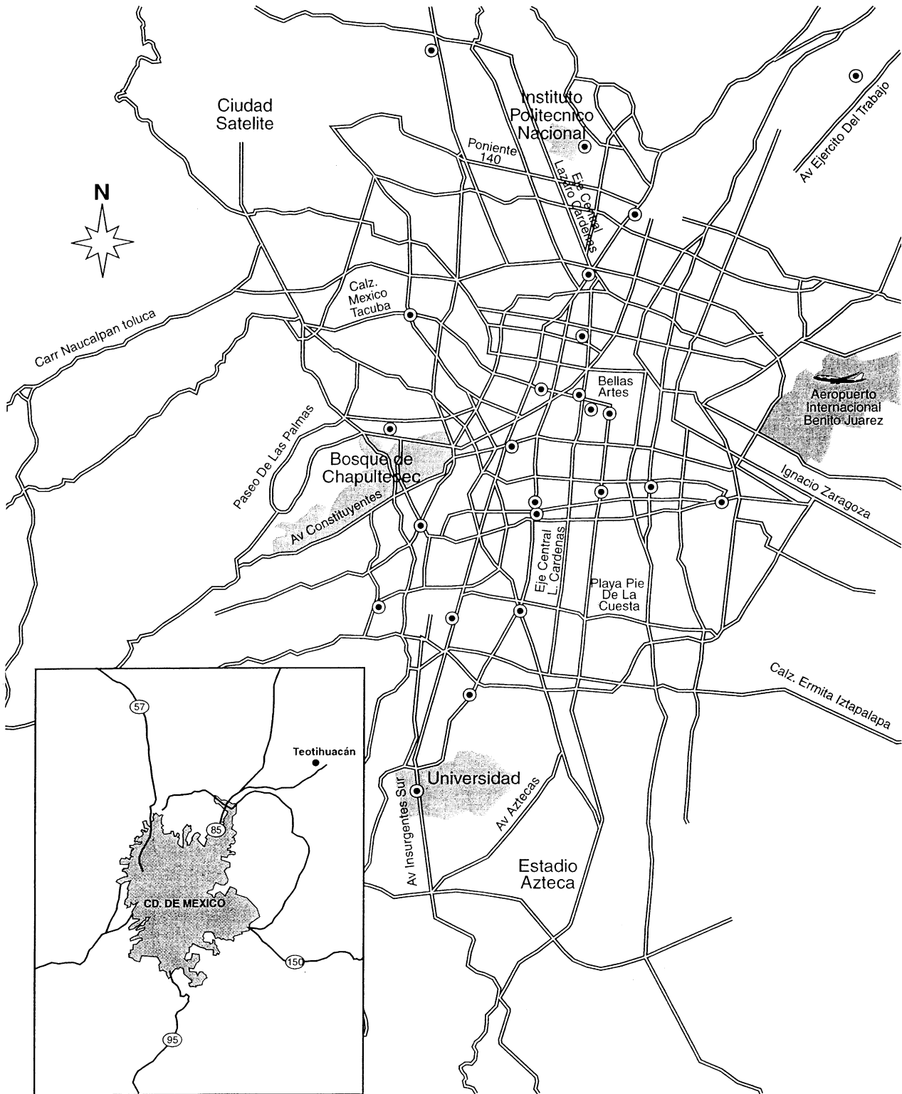
Fig. 1. Map of Mexico City and sampling localities. The urban area of Mexico City is located in a high elevation basin with several of the surrounding mountains exceeding 5000 m. The metropolitan area covers some 2500 km 2 and is occupied by ~20 million people. The ancient city of Teotihuacan, located some 60 km NE of the outskirts of Mexico City, was used as a baseline for comparisons. Levels there were comparable to baseline estimates at other locations around the globe (Blake et al., 1984; Houghton et al., 1996).
