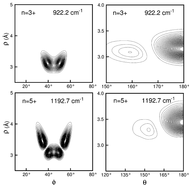
Figure 8. Contour plots of the probability density for the \psi_3^+ and \psi_5^+ states in hyperspherical Radau coordinates ( \phi , \rho ) at colinear geometry (left panel) and ( \theta , \rho ) for \phi = 45^\circ (right panel).
