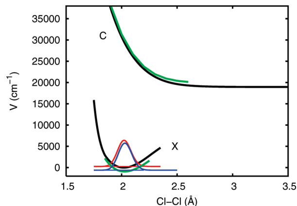
Figure 5. \text{Cl}_2 X and C curves without (black curves) or with (green curves) water at equilibrium distance. Also shown is the (X, v = 0 ) bound state wave function of \text{Cl}_2 without (red curve) or with (blue curve) water at equilibrium distance. The most important difference in the Franck–Condon region is the bound state energy. Note also the slight lengthening of the Cl–Cl bond upon dimer formation and the relative flattening of the C state repulsive wall in the Franck–Condon region.
