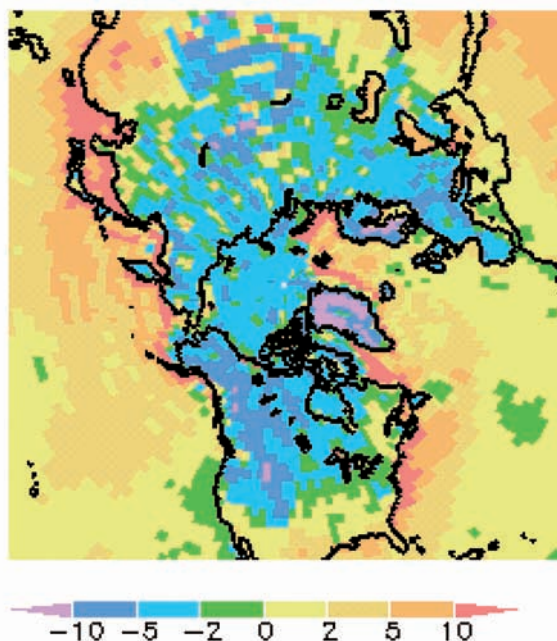
BL Diabatic Heating Rate(K/day), January
